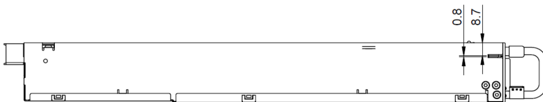
Figure 45 - Side View 2
